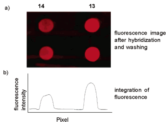
Figure 1. Fluorescence of spots of a DNA microarray after incubation at 70 °C with fluorescent complementary strand Cy3-ATCGCAGTCAACCA ( 15 ) and washing (a) Fluorescence image, with spots featuring control strand 14 (left) and 3'-capped strand 13 (right). Spotting was in duplicate to demonstrate reproducibility. (b) Integration of fluorescence over the area vertically above.
